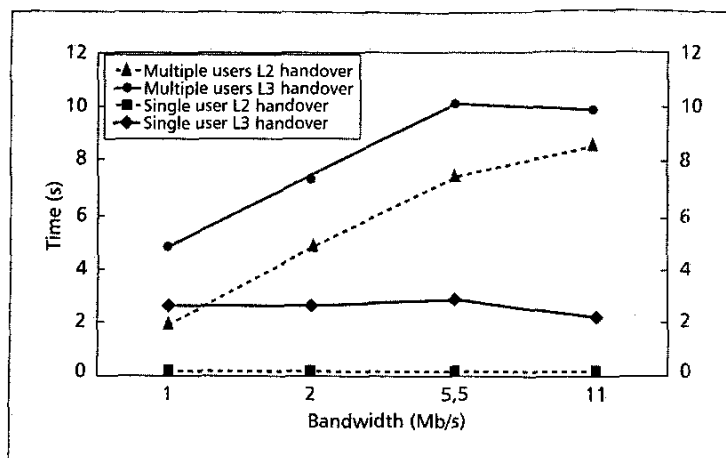
Figure 5. L2 and L3 handover latencies.
