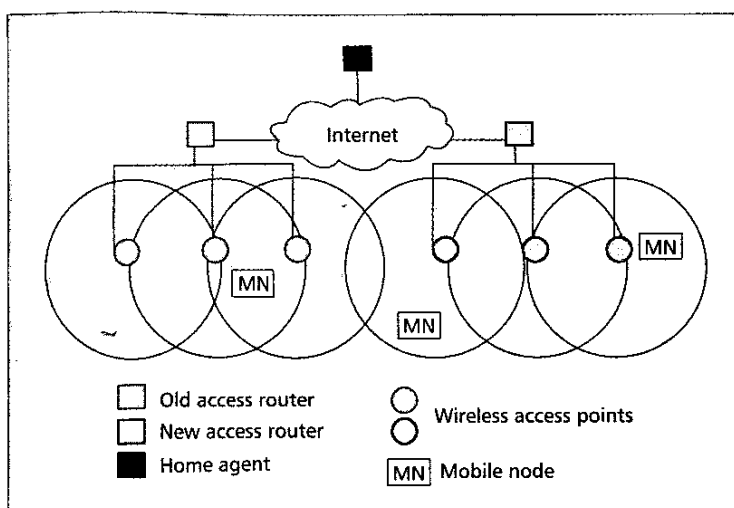
Figure 1. IPv6 wireless network architecture.
