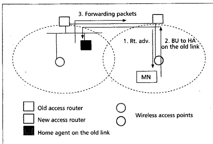
Figure 2. Forwarding from the old access network.
