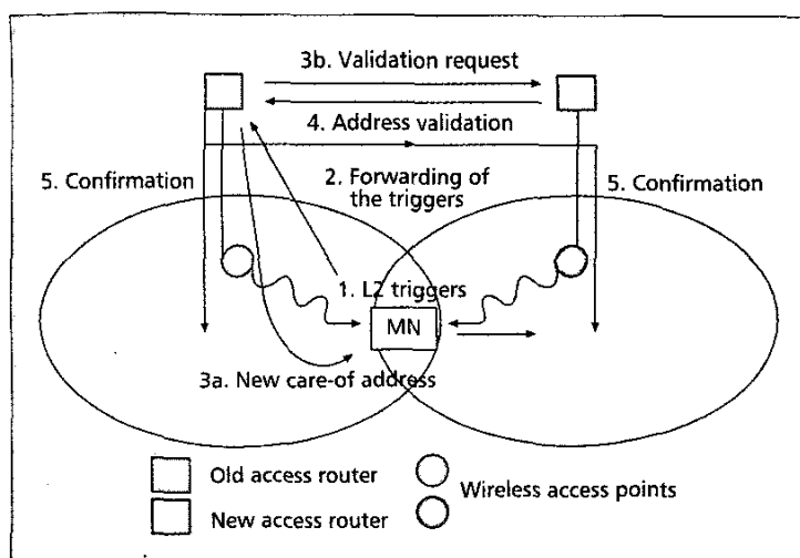
■ Figure 4. Anticipated handover.
